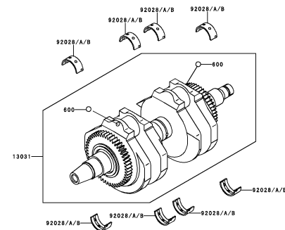
B-12 Crankshaft
