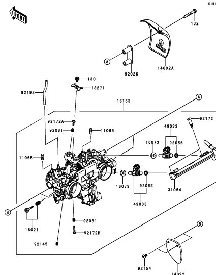
C-11 Throttle
