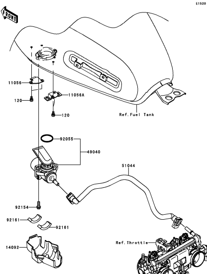
C-12 Fuel Pump
