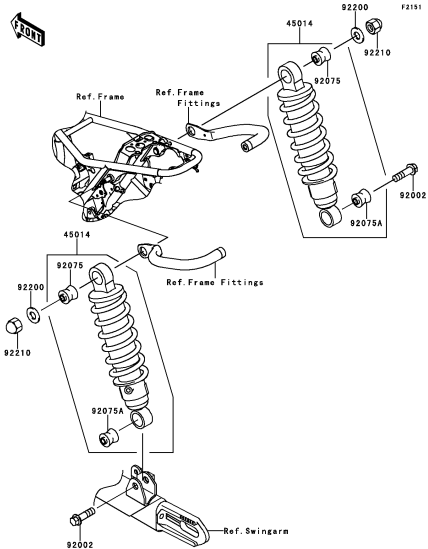
E-7 Suspension/Shock Absorber
