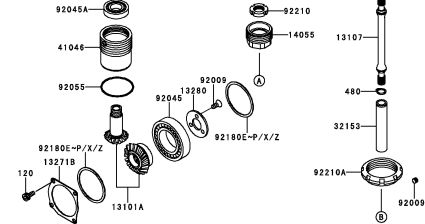
B-10 Camshaft(s)/Bevel Gear(1/2)
