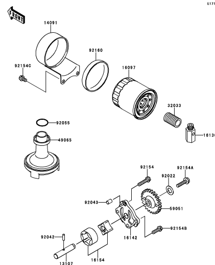
C-14 Oil Pump
