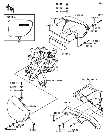
F-11 Side Covers/Chain Cover
