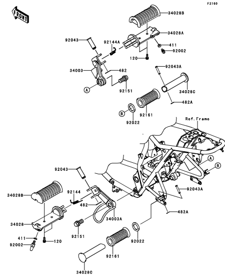
E-8 Footrests
