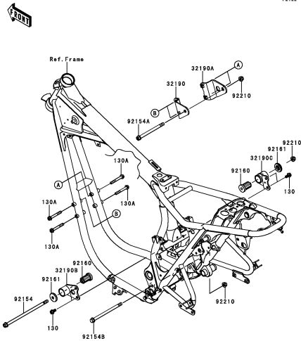
E-4 Engine Mount
