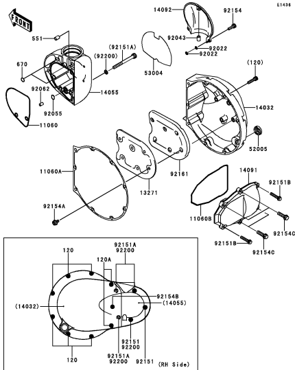
C-10 Right Engine Cover(s)
