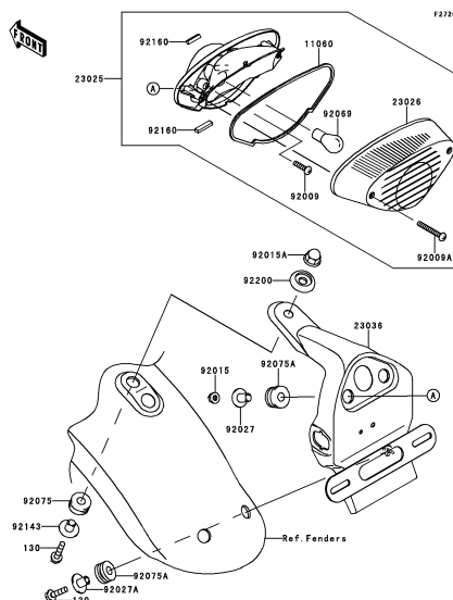
F-13 Taillight(s)
