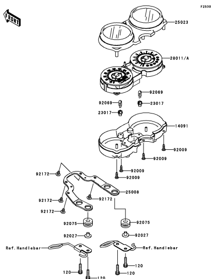
F-9 Meter(s)
