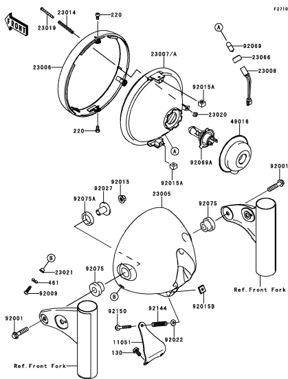
F-12 Headlight(s)
