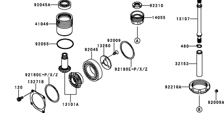
B-11 Camshaft(s)/Bevel Gear(2/2)
