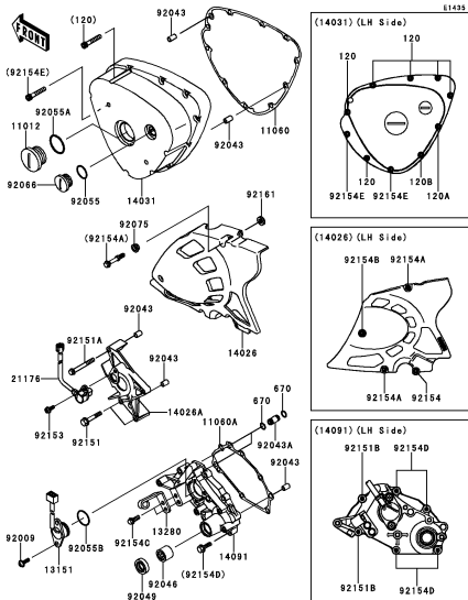
C-9 Left Engine Cover(s)
