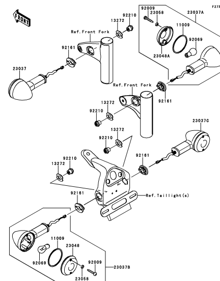
F-14 Turn Signals
