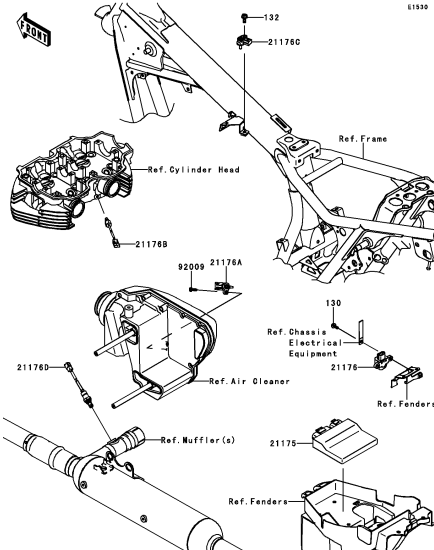
C-13 Fuel Injection
